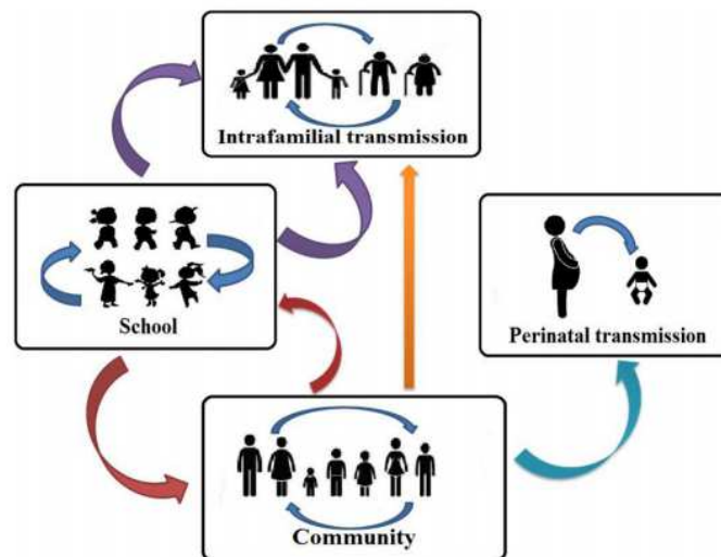
Figure 3: Transmission dynamics of SARS-CoV-2 infection in People
