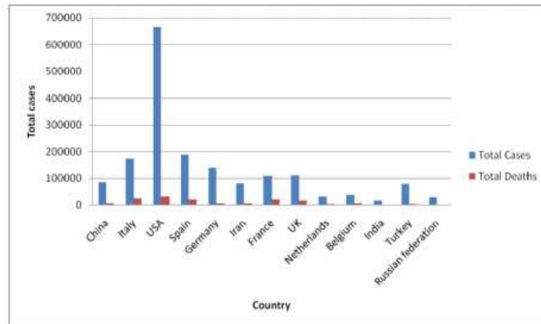
Figure 1: The comparative study of COVID-19 cases of USA with other Country (WHO, 2020).
